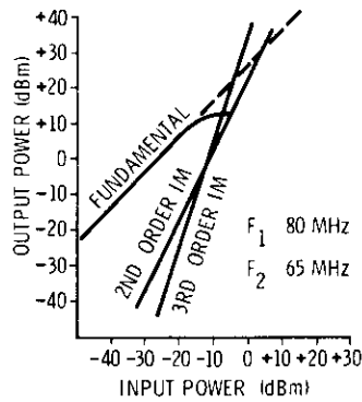
Intermodulation Intercept Points
